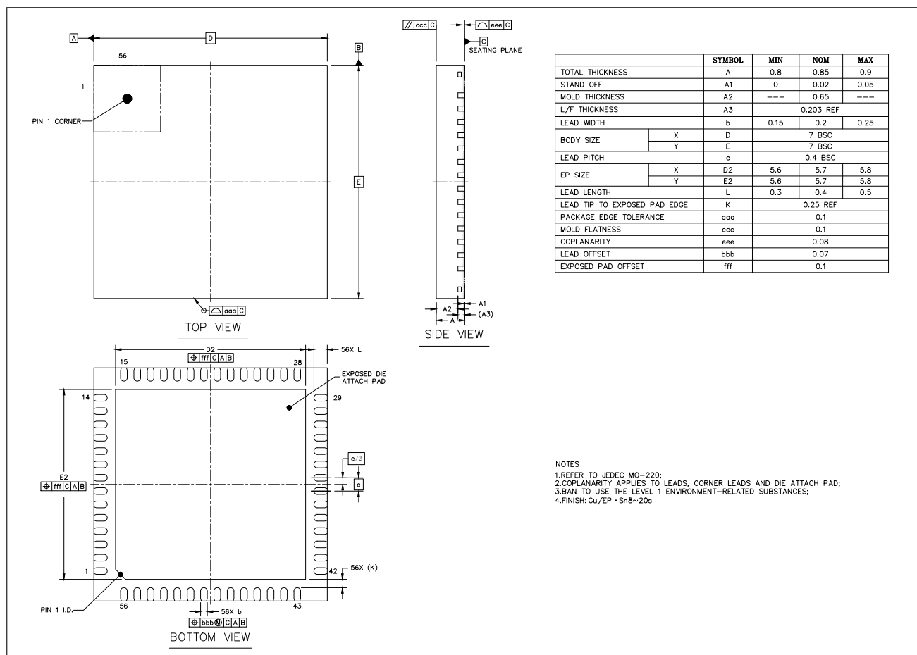
Figure 7-2. QFN56 (7x7 mm) Package (Only for ESP32-S3FH4R2)
